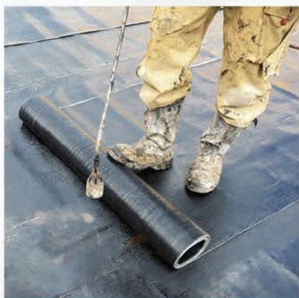
Bitumen Membrane Waterproofing
